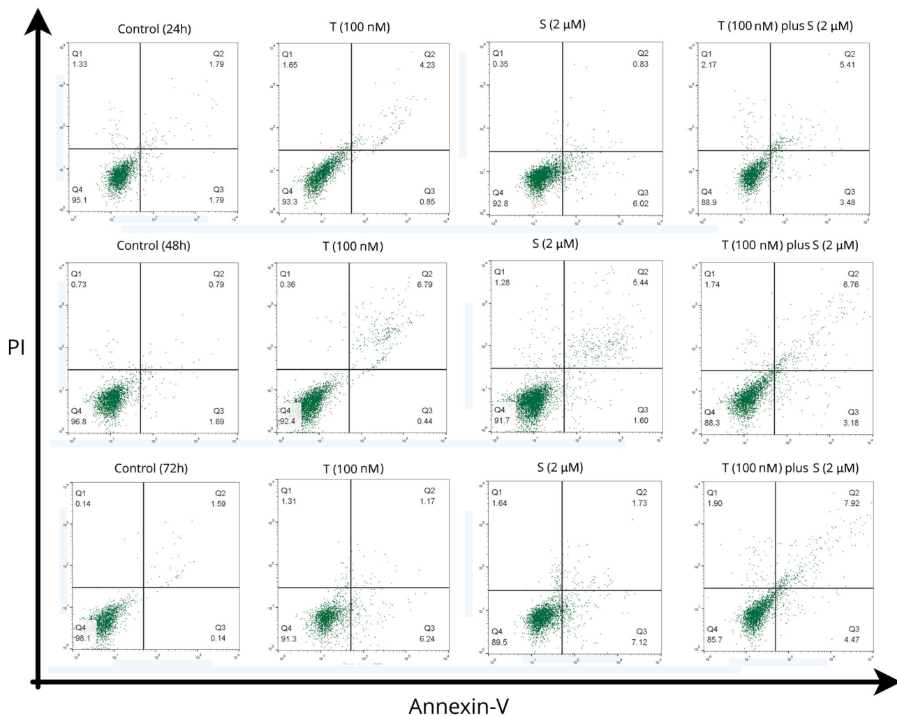
Fig. 2 Apoptosis of the HEK-293 cells treated with TRAIL (100 nM) and SAHA (2 \mu M) separately and together after 24, 48, and 72 h of exposure. Following Annexin-V and PI staining, cell death was calculated using FACS analysis, as detailed in the “materials and methods”
