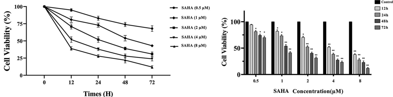
Fig. 1 The cytotoxic effect of SAHA on K562 cell proliferation. After exposure to different concentrations of SAHA (0–8 \mu M) for 12, 24, 48, and 72 h, the IC 50 values in K562 cells were calculated by applying
